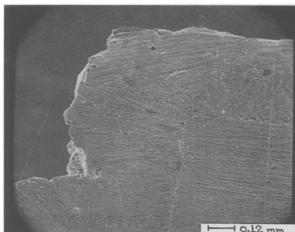
Fig. 12. SEM micrograph of the molybdenum coating of Fig. 11, showing uniformity of thickness around a right angle bend.
