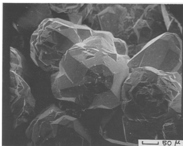
Fig. 4. Surface of molybdenum deposit of Fig. 2.
