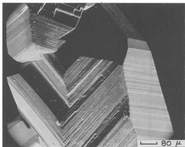
Fig. 6. SEM micrograph of the tip of the needles of the deposit shown in Fig. 5.
