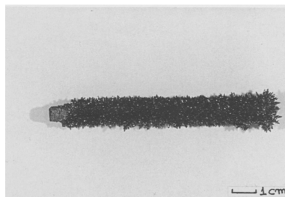
Fig. 5. Molybdenum deposit on a graphite substrate. Electrolyte composition (ii). Current density 300 \text{ A m}^{-2} . Temperature 800^\circ \text{C} . Experiment iia.
