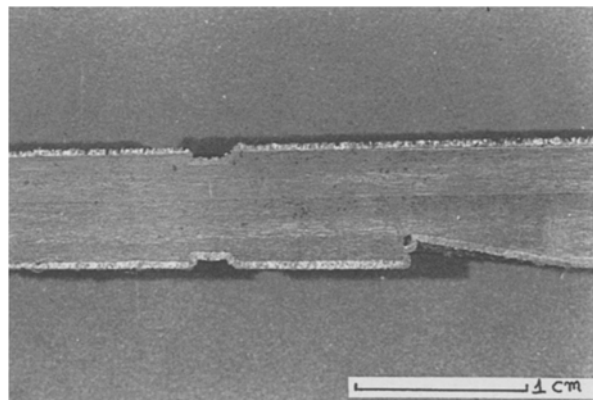
Fig. 11. Longitudinal section of the specimen of Fig. 10 showing excellent throwing power.
