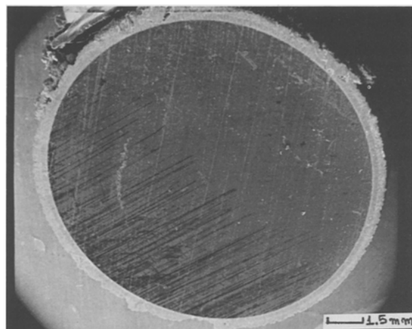
Fig. 2. SEM micrograph of a molybdenum deposit on a graphite substrate. Electrolyte composition (i). Current density 500 \text{ A m}^{-2} . Temperature 800^\circ \text{C} . Experiment ib.
