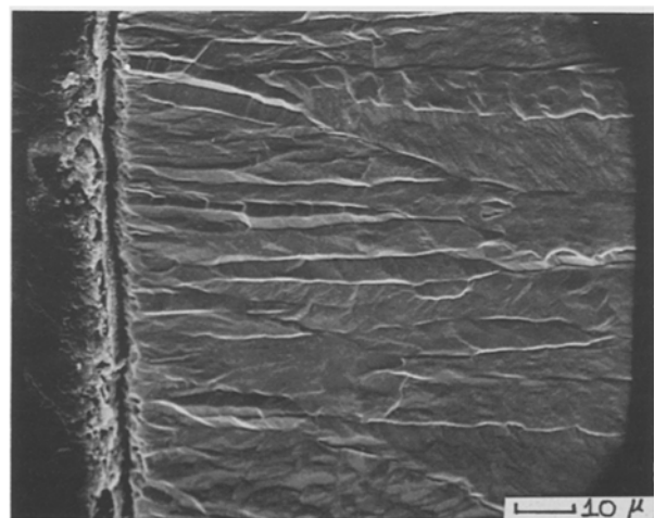
Fig. 3. SEM micrograph of molybdenum deposit of Fig. 2 showing characteristic columnar structure.
