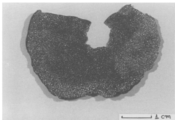
Fig. 7. Plate-like molybdenum deposit grown on the surface of the electrolyte. Experiment iia.
