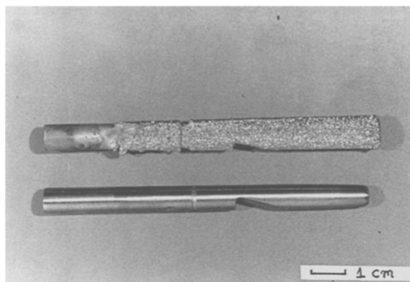
Fig. 10. Specimen for testing the throwing power of the electrolyte. Electrolyte composition (iii), 1.8% \text{Al}_2\text{O}_3 . Current density 330 \text{ A m}^{-2} . Temperature 800^\circ\text{C} . Electroplated specimen (top), machined and polished substrate before plating (bottom).
